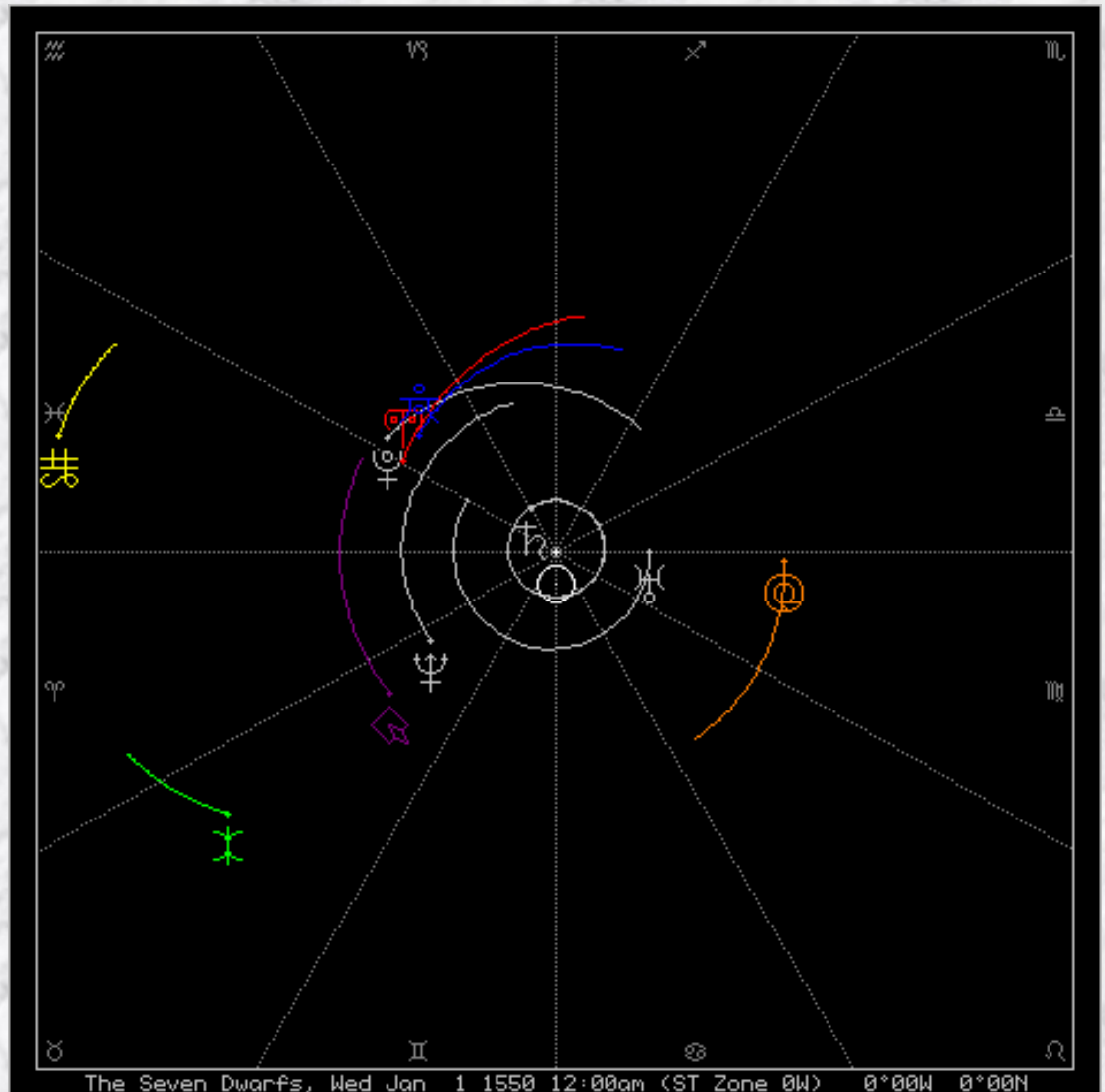
Above: Orbits of the Seven Dwarfs.
